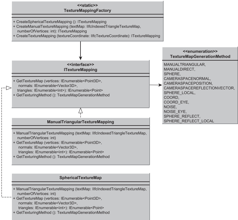
Figure 4.17: UML diagram of the structure for texture maps.
